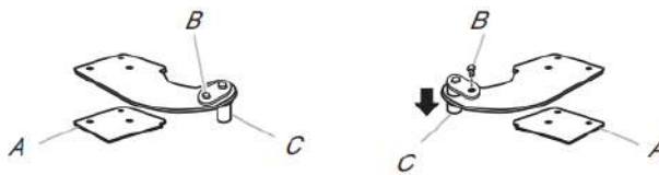
A. Plastic spacer B. Hinge pin screw C. Hinge pin
